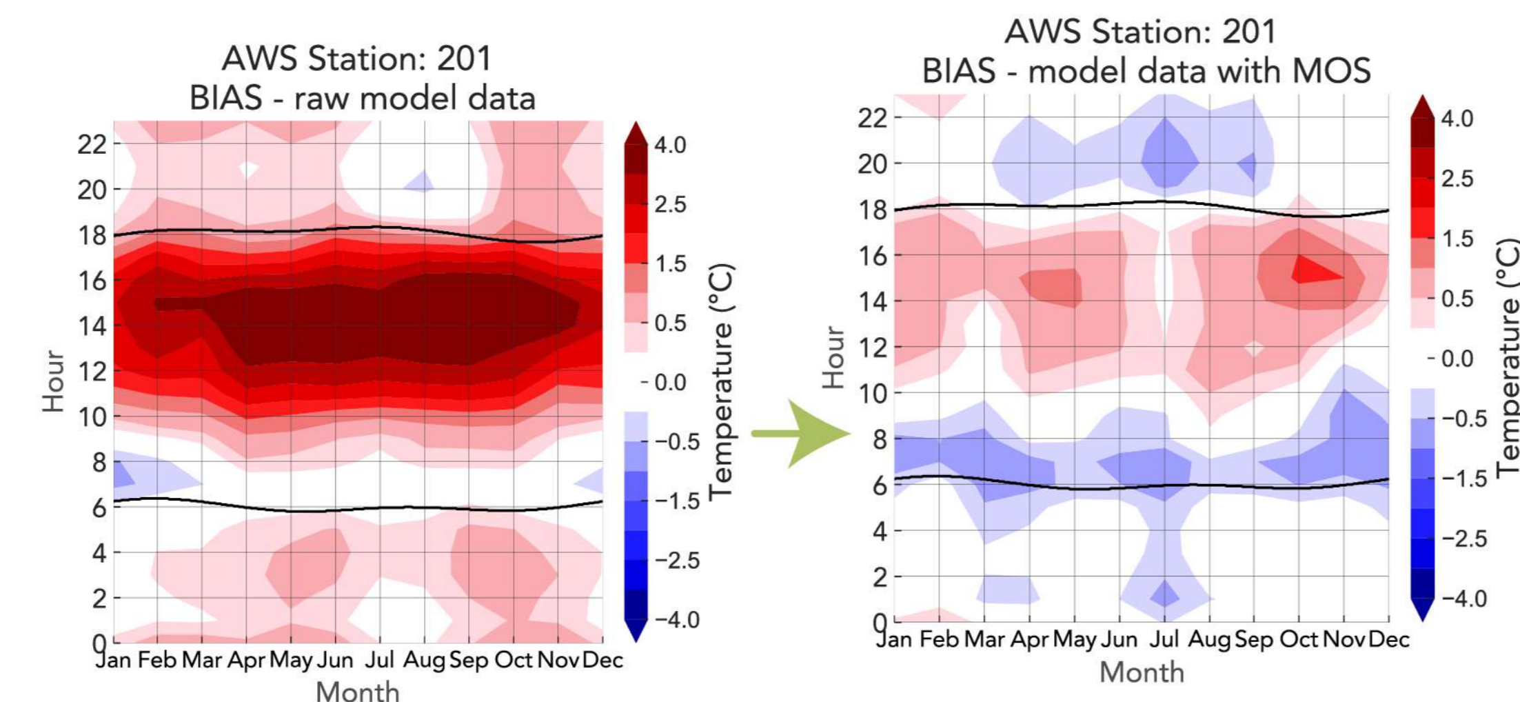
Monthly diurnal cycle of temperature differences between forecast and observations with and without MOS
