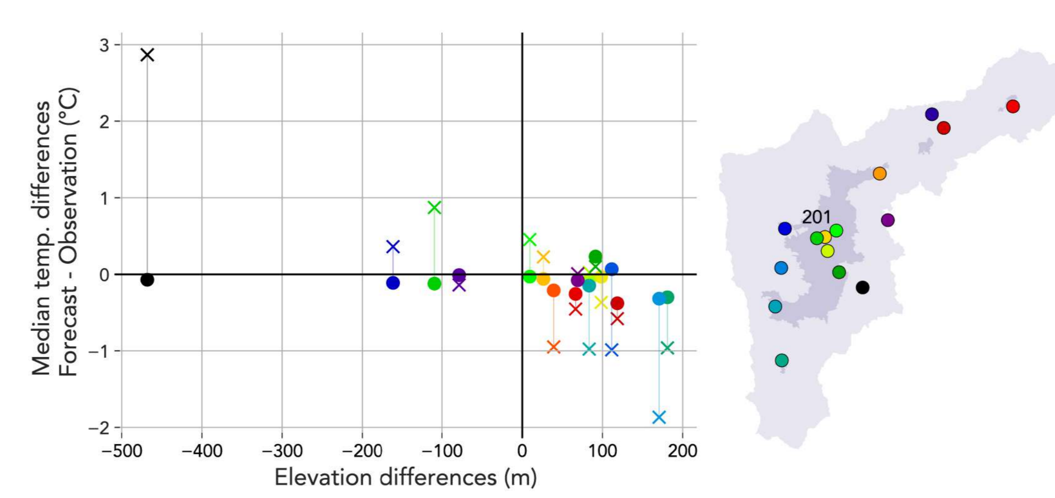
Elevation differences vs. temperature differences Crosses (points) indicate temperature differences before (after) MOS.
