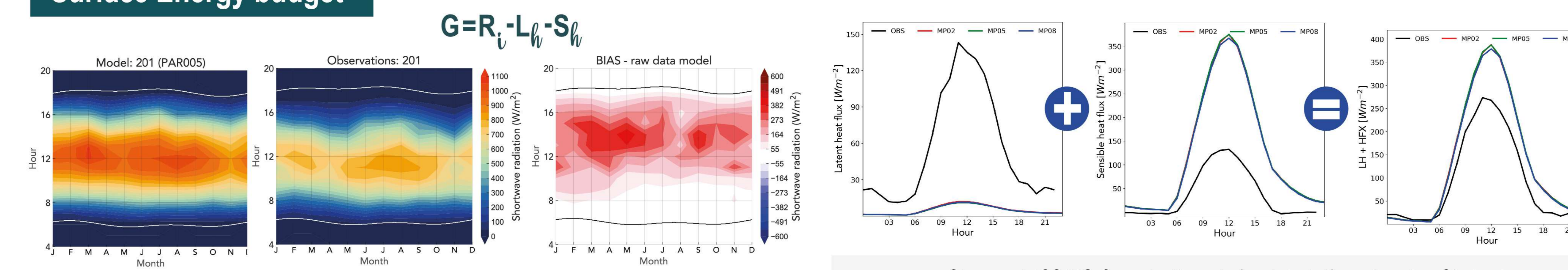
Observed, simulated and differences of surface radiation (land use = Urban)
