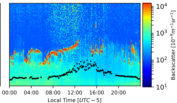
03-04-2015 Richardson Number Retrievals
