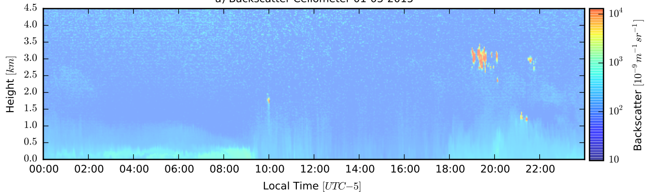
a) Backscatter Ceilometer 01-03-2015
