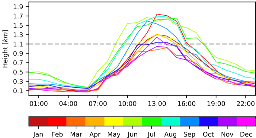
ABL Monthly Diurnal Cycle - Param 8 - Day 3 - AMVA
