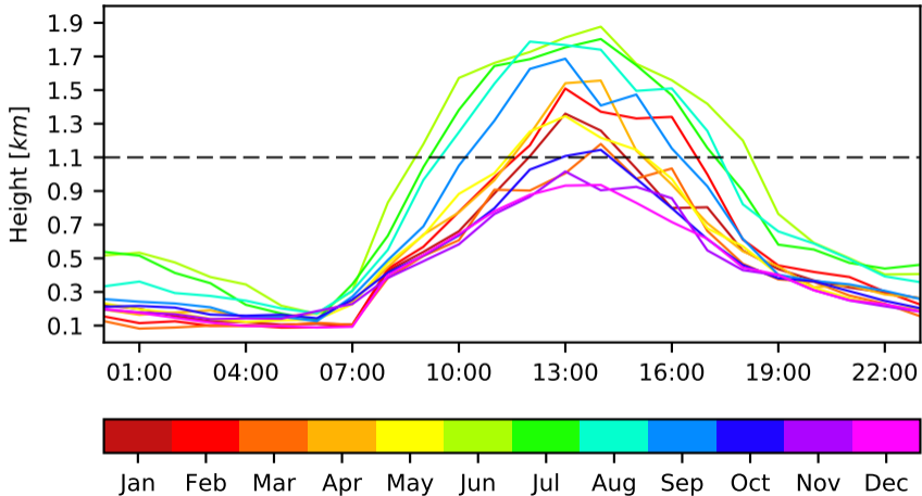
ABL Monthly Diurnal Cycle - Param 8 - Day 2 - SIATA
