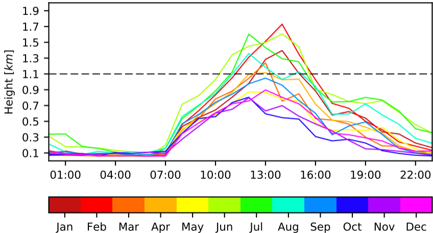
ABL Monthly Diurnal Cycle - Param 8 - Day 2 - Itagui
