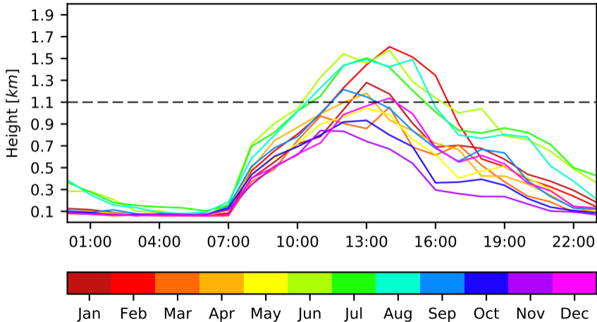
ABL Monthly Diurnal Cycle - Param 8 - Day 1 - Itagui
