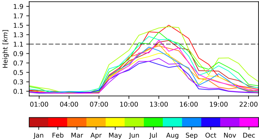
ABL Monthly Diurnal Cycle - Param 5 - Day 3 - Itagui
