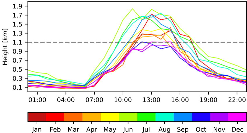
ABL Monthly Diurnal Cycle - Param 5 - Day 3 - AMVA
