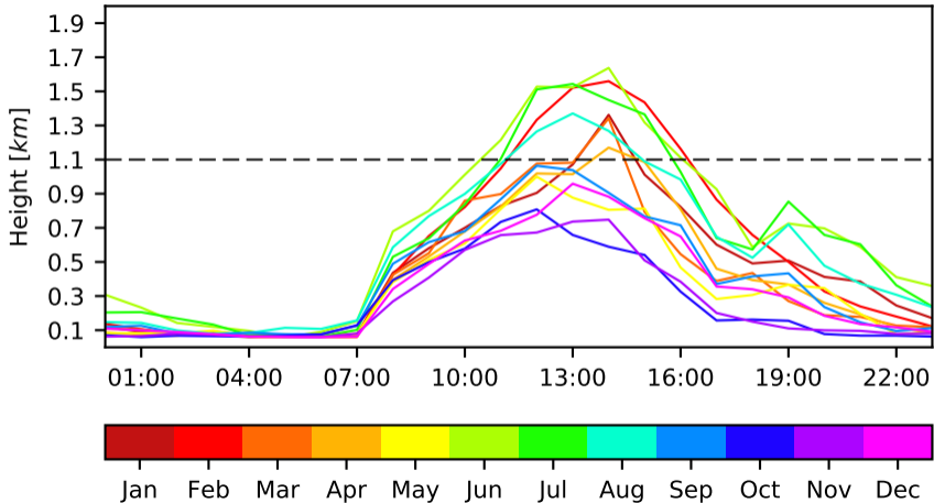
ABL Monthly Diurnal Cycle - Param 5 - Day 2 - Itagui
