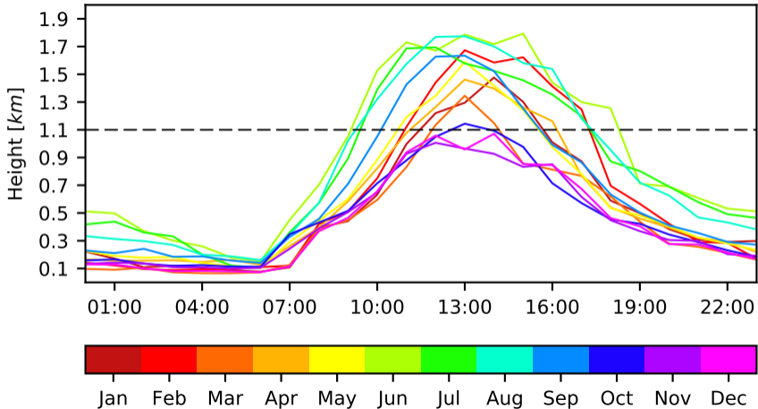
ABL Monthly Diurnal Cycle - Param 5 - Day 2 - AMVA
