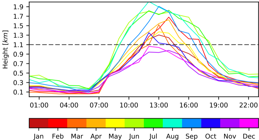
ABL Monthly Diurnal Cycle - Param 5 - Day 1 - SIATA
