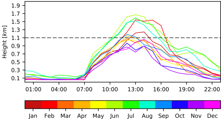
ABL Monthly Diurnal Cycle - Param 5 - Day 1 - Itagui
