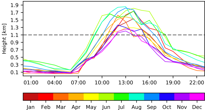
ABL Monthly Diurnal Cycle - Param 5 - Day 1 - AMVA
