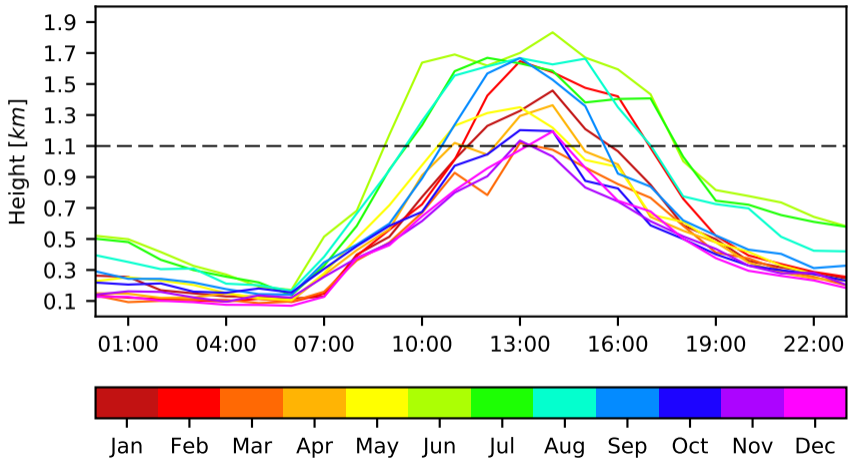
ABL Monthly Diurnal Cycle - Param 2 - Day 3 - AMVA
