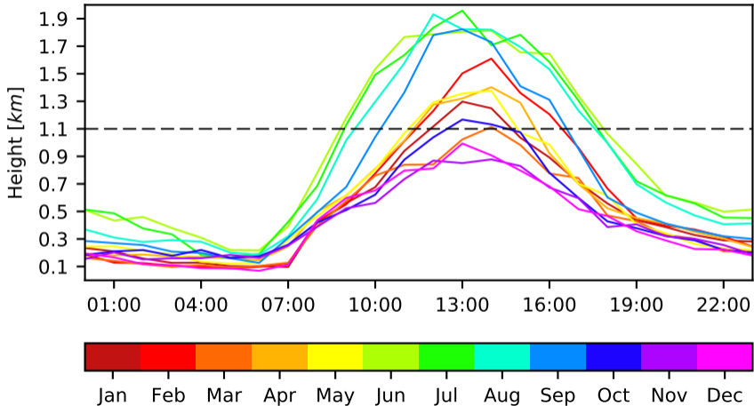
ABL Monthly Diurnal Cycle - Param 2 - Day 2 - SIATA
