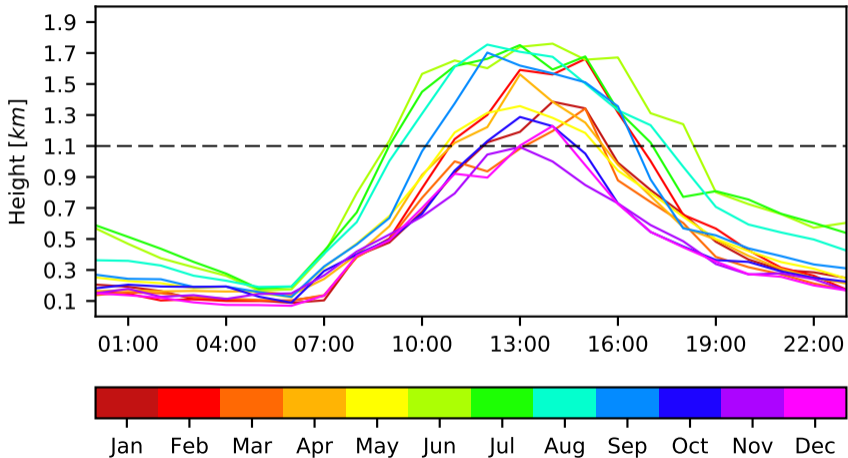
ABL Monthly Diurnal Cycle - Param 2 - Day 2 - AMVA
