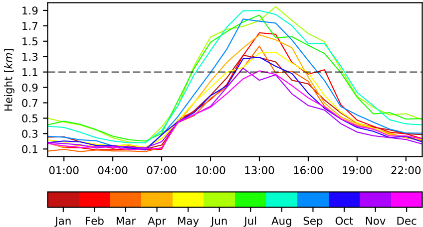
ABL Monthly Diurnal Cycle - Param 2 - Day 1 - SIATA
