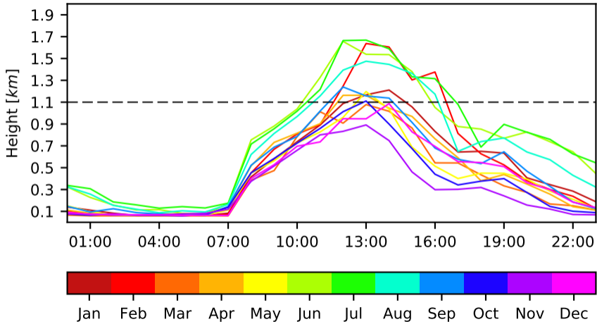
ABL Monthly Diurnal Cycle - Param 2 - Day 1 - Itagui
