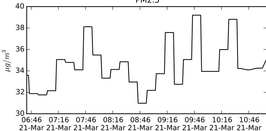
PM2.5
