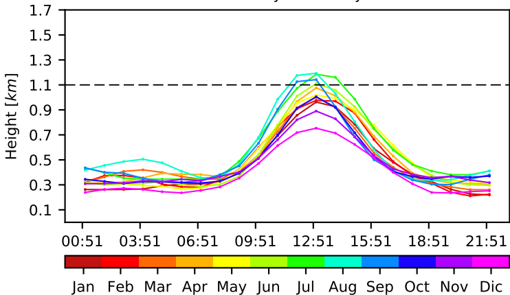
ABL Monthly Diurnal Cycle
