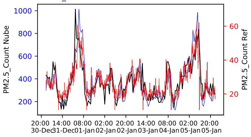
PM2.5_Count
